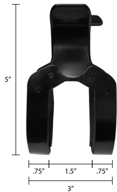
Large Claw
